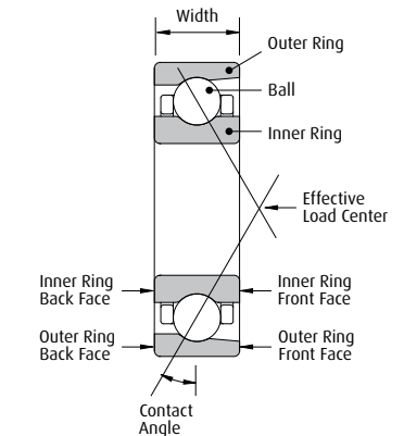
Single Row Angular Contact Ball Bearing
