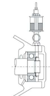
Drip Feed Lubrication: for high speeds
