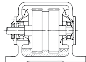
Splash Lubrication: gearboxes
