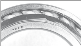
Fig. 1: Grease Packed Angular Contact Ball Bearing
