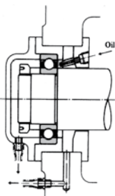
Jet Lubrication: ultra high speeds, like jet engine or machine tool spindles
