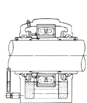
Oil Bath Lubrication: not for high speeds
