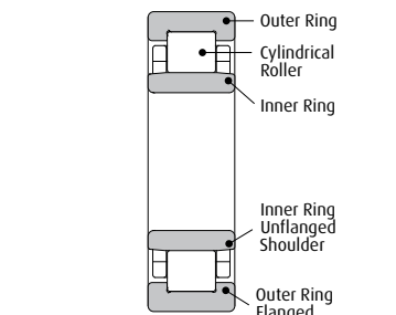
Cylindrical Roller Bearing (NU Style)
