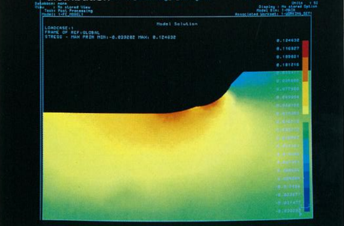
Fig. 7 An example of FEM analysis of shaft stress distribution
