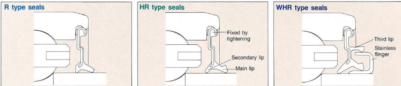
Fig. 1 Kinds of seals
