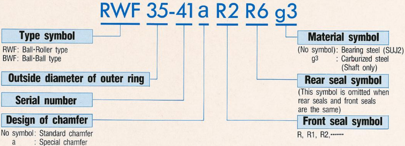
Fig. 13 Formulation of bearing numbers
