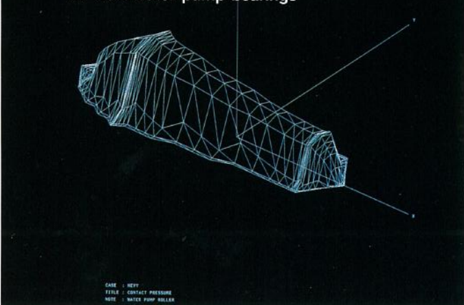
Fig. 6 Distribution of roller surface pressure for NSK water pump bearings
