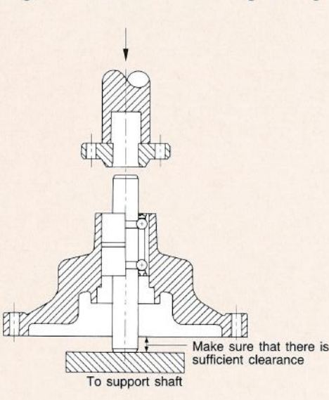
Fig. 12 Pressing hub onto shaft of mounting bearing
