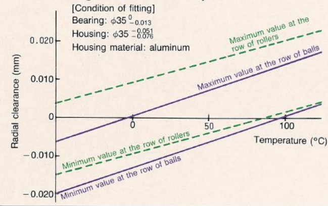
Fig. 10 Water pump bearings: correlation of internal bearing clearance and temperature
