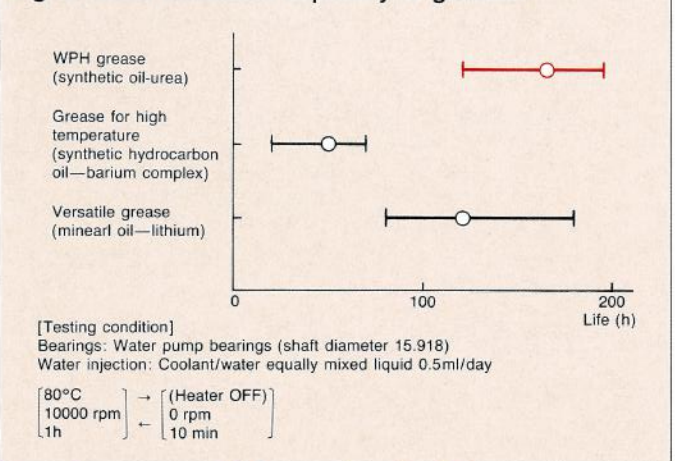
Fig. 3 Water resistance capability of greases
