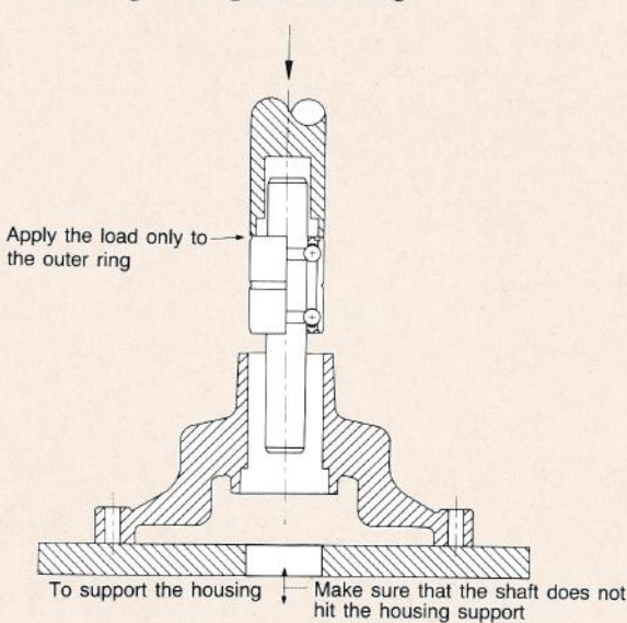
Fig. 11 Pressing bearing into housing
