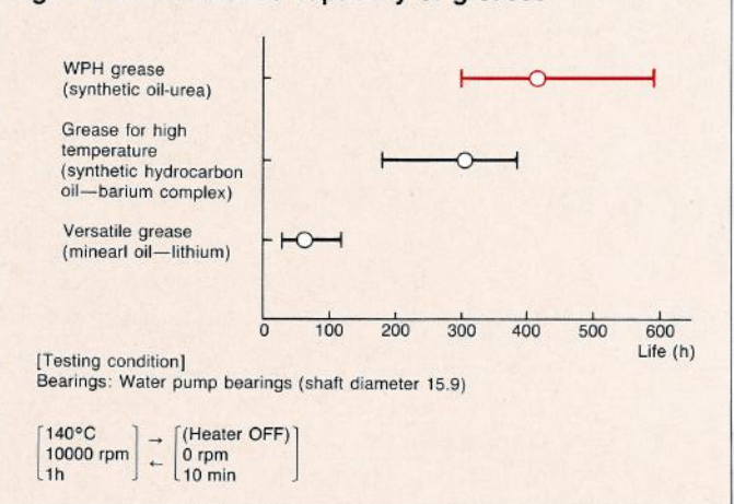
Fig. 4 Heat resistance capability of greases
