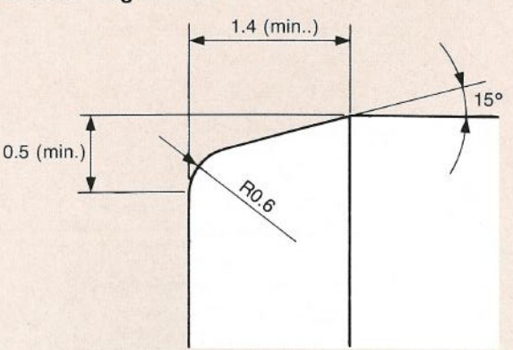
Fig. 9 Outer ring chamfer
