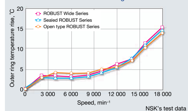
Comparison of temperature rise between open type and sealed bearings
